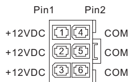
+12V PCI Express Connector
