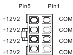
Main power connector
