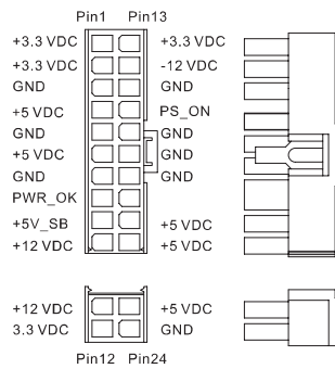
Main power connector
