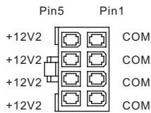
+12V power connector
