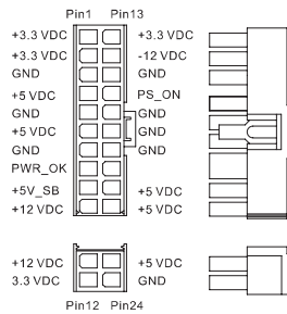
Main power connector
