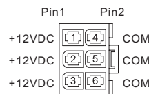
+12V PCI Express Connector
