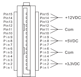
Serial ATA power connector
